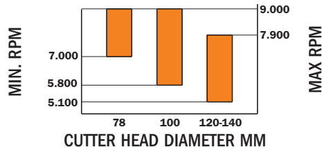
SUGGESTED CUTTER HEADS ROTATION
